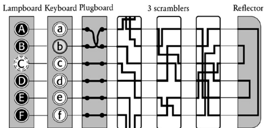
Figure 37 The plugboard sits between the keyboard and the first scrambler. By inserting cables it is possible to swap pairs of letters, so that, in this case, b is swapped with a. Now, b is encrypted by following the path previously associated with the encryption of a. In the real 26-letter Enigma, the user would have six cables for swapping six pairs of letters.
