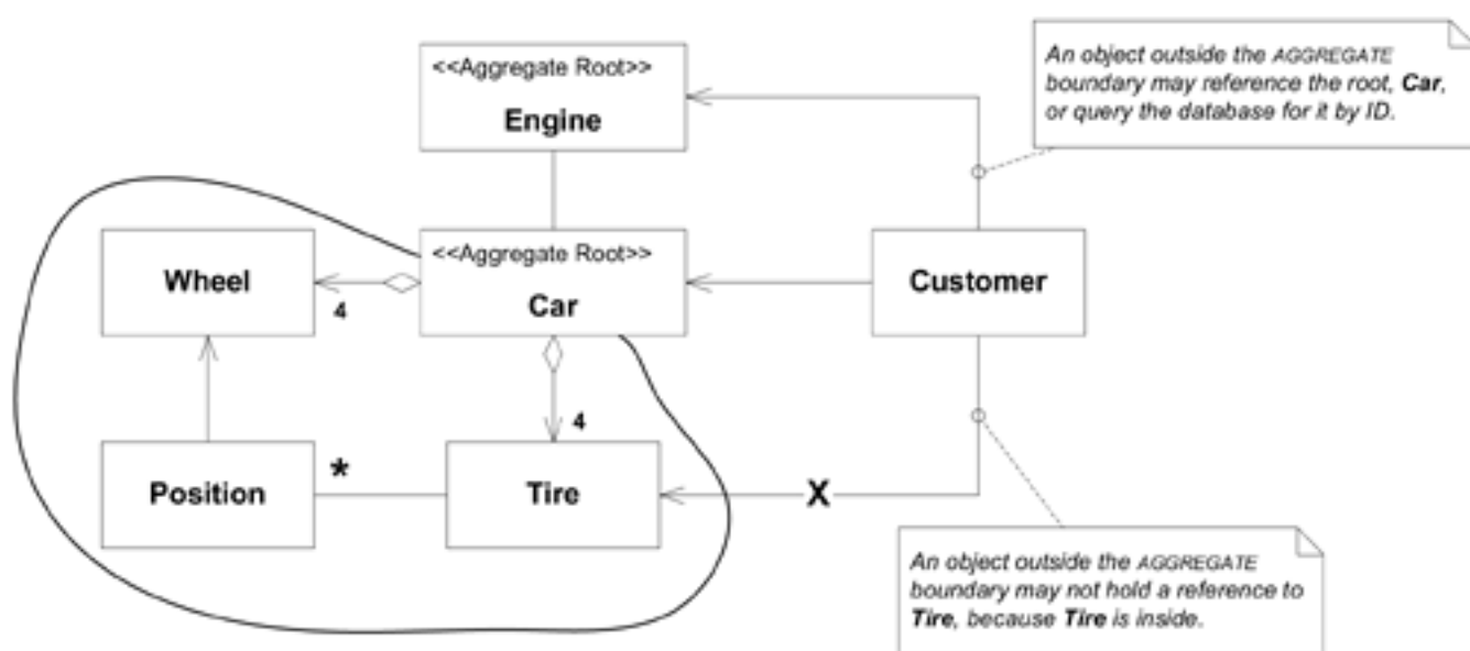
Figure 6.2. Local versus global identity and object references
