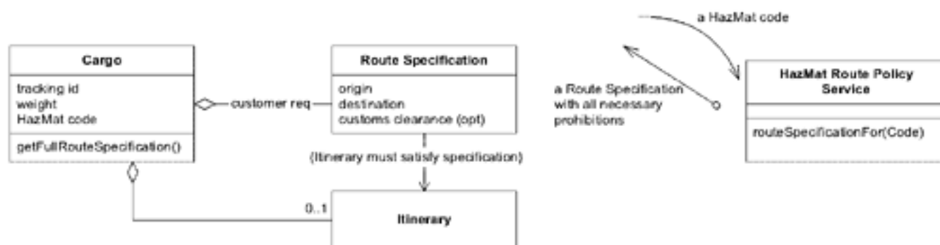
Figure 16.9. A possible design for routing hazardous cargo
