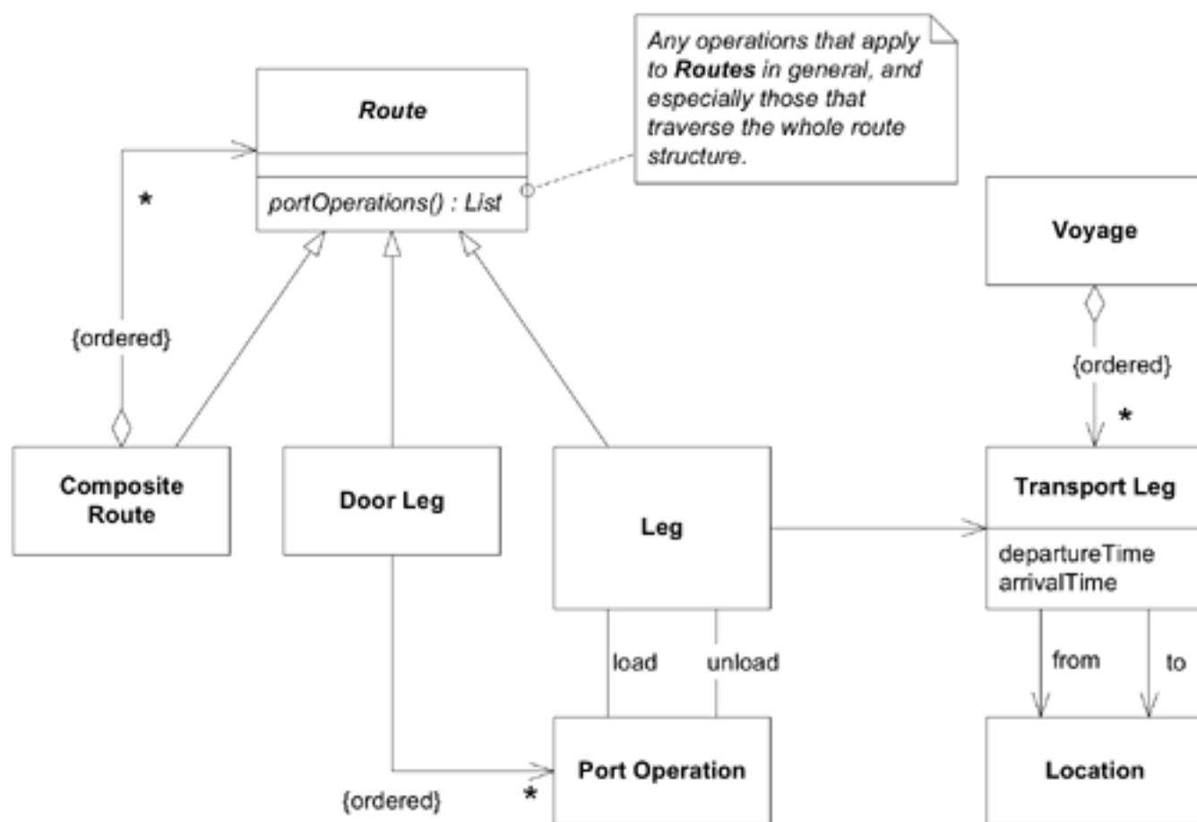
Figure 12.8. A class diagram using COMPOSITE
