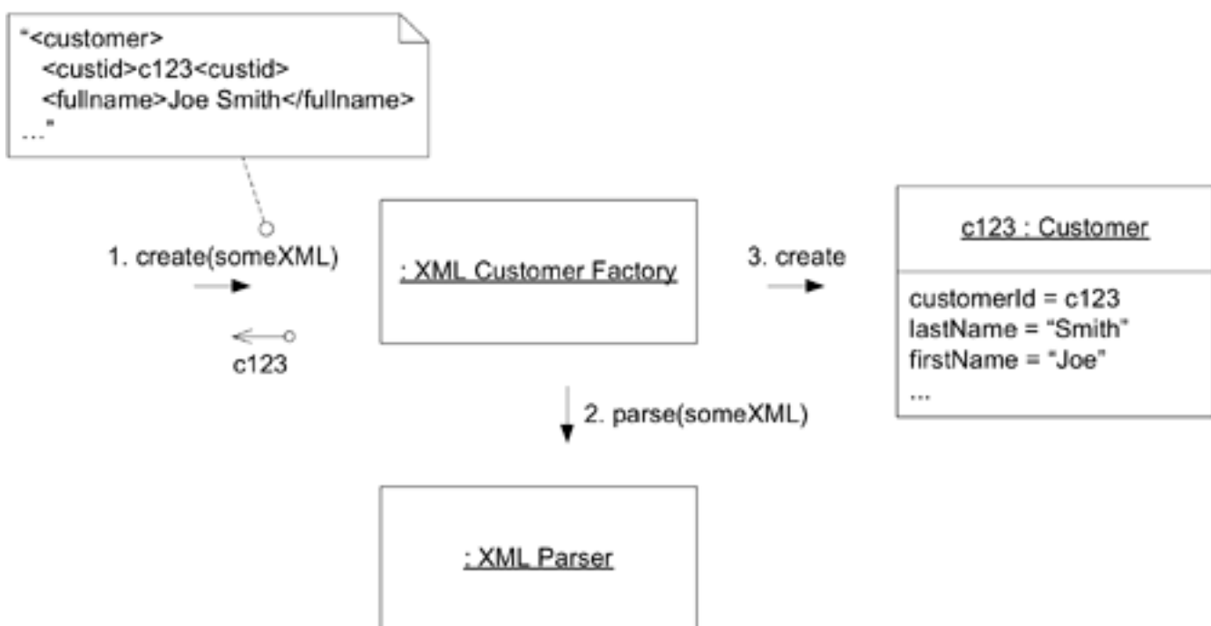
Figure 6.17. Reconstituting an ENTITY transmitted as XML
