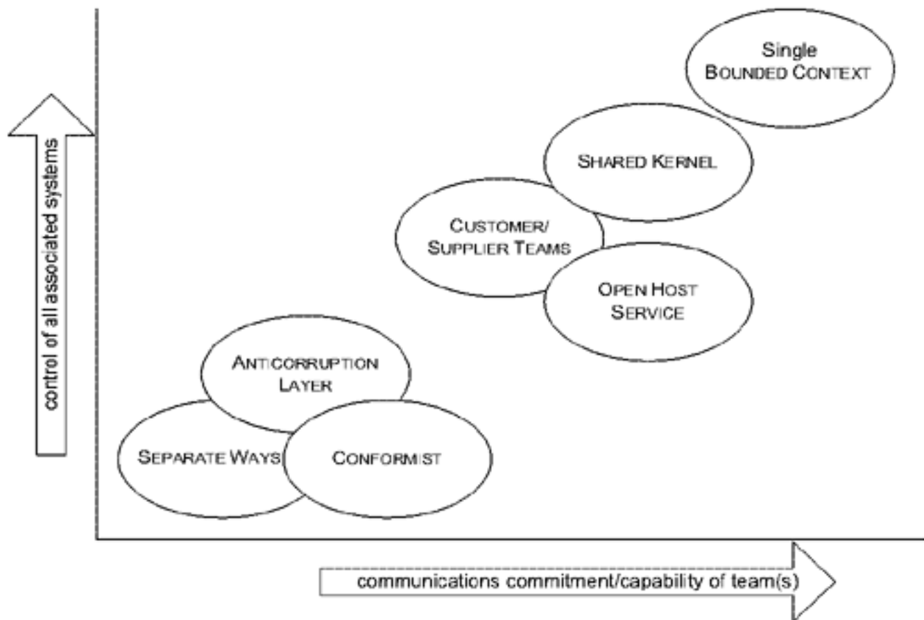
Figure 14.13. The relative demands of CONTEXT relationship patterns
