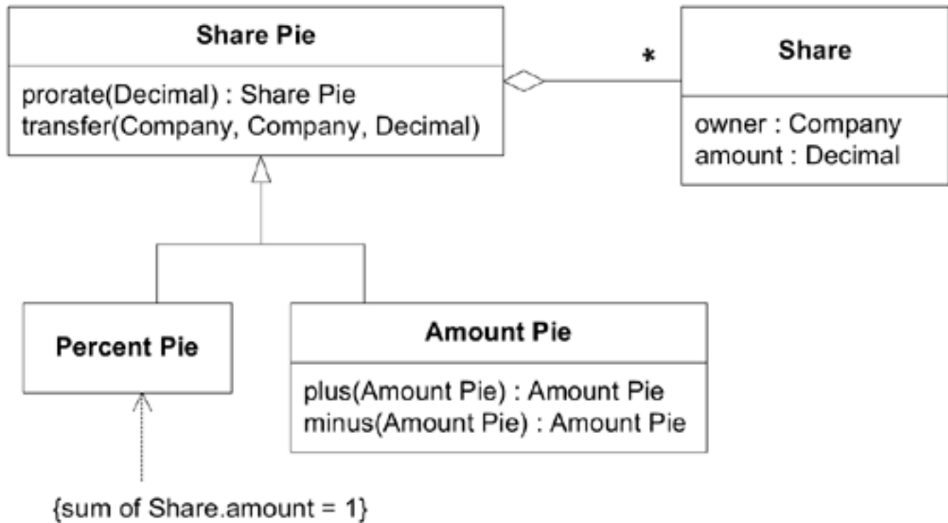
Figure 8.7. An abstract model of shares
