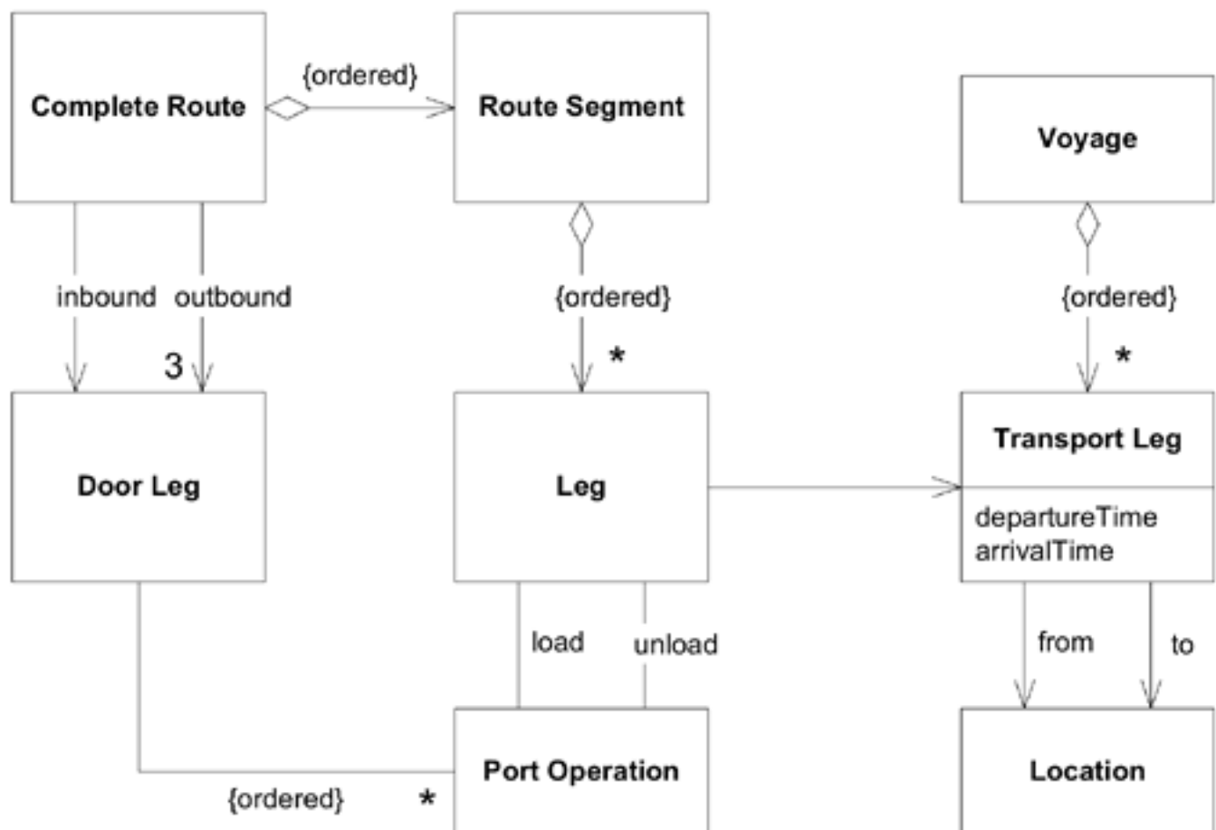
Figure 12.7. The elaborated class diagram of Route
