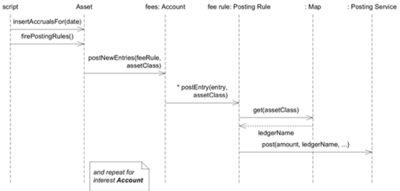
Figure 11.11. Sequence diagram showing rule firing
