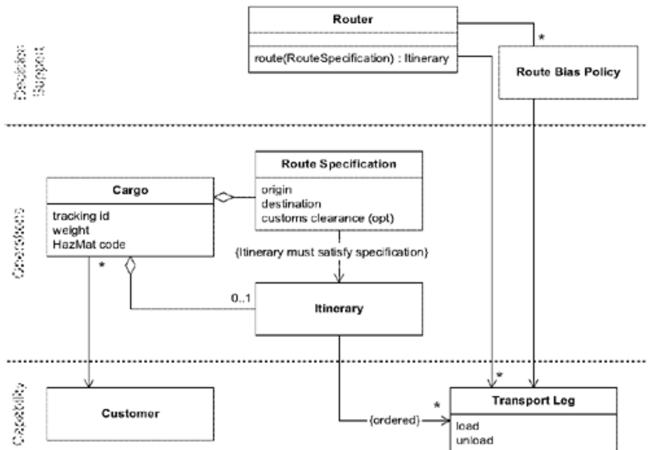
Figure 16.8. The restructured and refactored model
