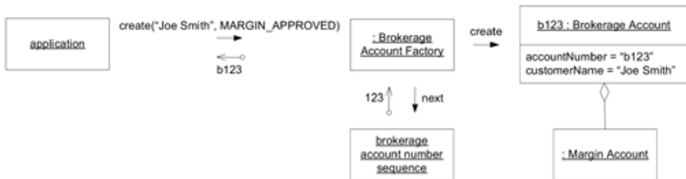
Figure 6.15. A standalone FACTORY builds AGGREGATE .
