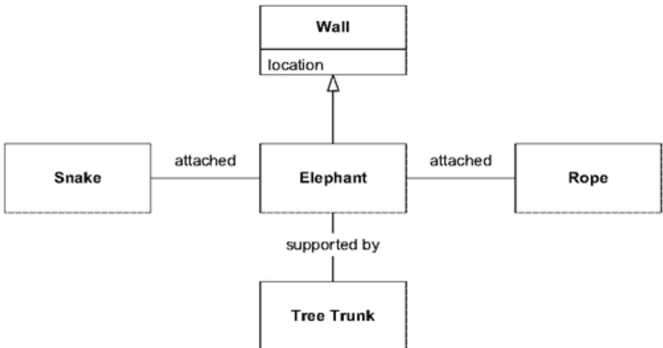
Figure 14.11. One context: crude integration
