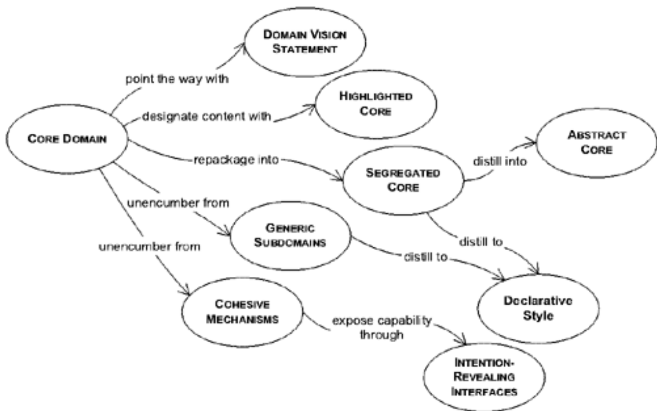
Figure 15.1. A navigation map for strategic distillation
