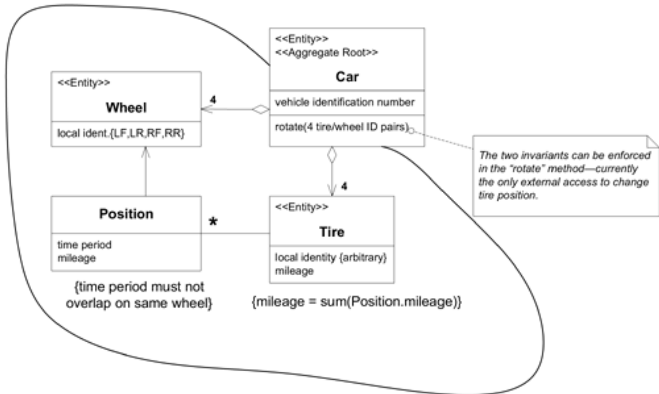
Figure 6.3. A GGREGATE invariants
