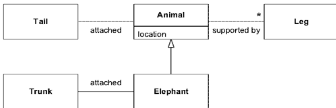
Figure 14.12. One context: deeper model
