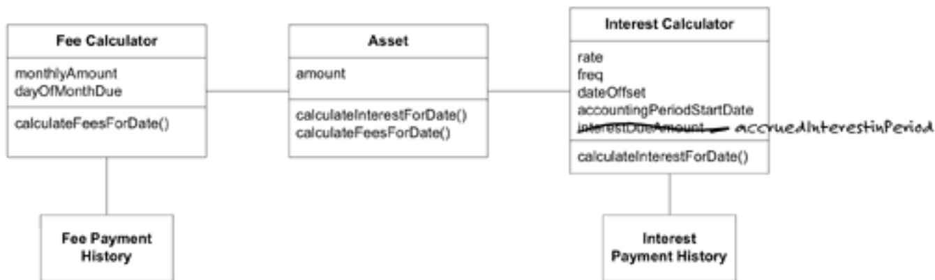
Figure 11.5. Original class diagram, accruals separated from payment
