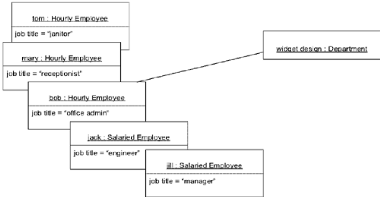
Figure 16.16. Some employees represented using the old model
