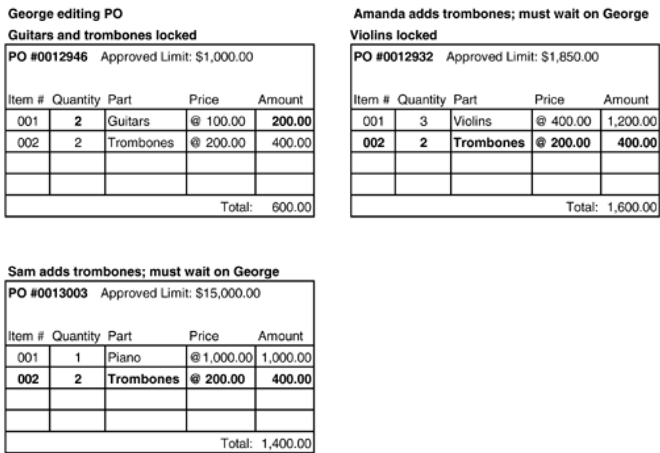
Figure 6.9. Over-cautious locking is interfering with people's work.
